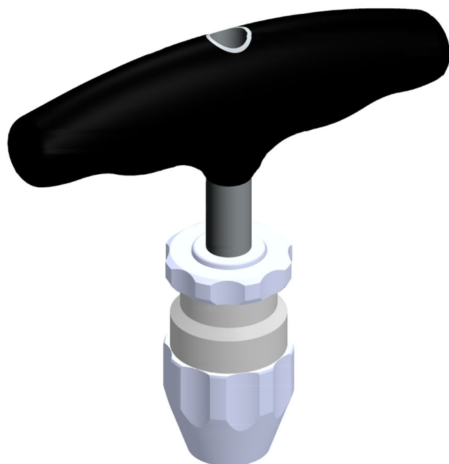
OM 19-0625 T23 Handle Speed Chuck 0.6-7.4mm Capacity Cannulated 115.3mm Height
