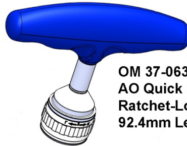
OM 35-0940 Q29 Handle Low Profile AO Quick Connect Ratcheting, Cannulated 100.8mm Length
