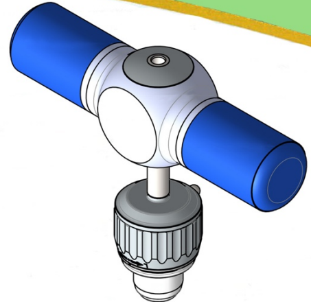
OM 31-0045 T28 Handle 1/4" Square Connect Ratcheting, Cannulated Torque Limiting 102.7mm Length
