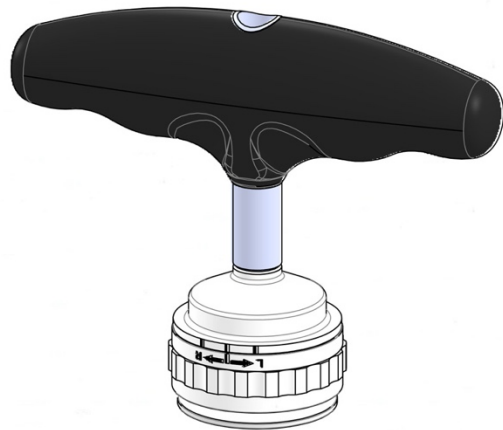
OM 37-0890 T23 Handle 1/4" Square Connect Ratcheting, Low Profile Release Cannulated 93mm Length
