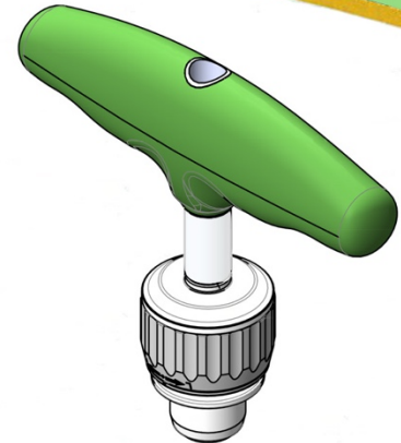
OM 22-0460 T23 Handle 1/4" Square Connect Ratcheting, Cannulated 104mm Length
