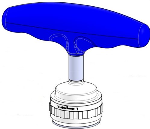
OM 37-0890 T23 Handle 1/4" Square Connect Ratcheting, Low Profile Release 92.9mm Length
