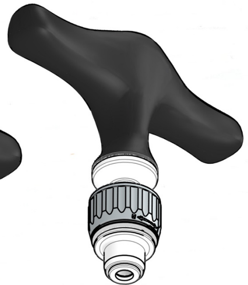
OM 37-0105 T33 Handle 1/4" Square Connect Ratcheting Torque Limiting - 8Nm 125.9mm Length
