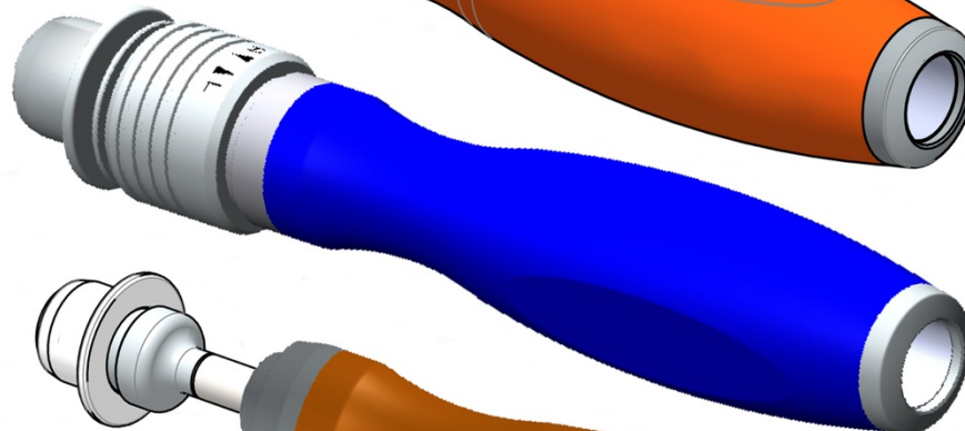
OM 13-0880 D23 Handle 1/4" Square Connect Ratcheting, Cannulated 165.6mm Length
