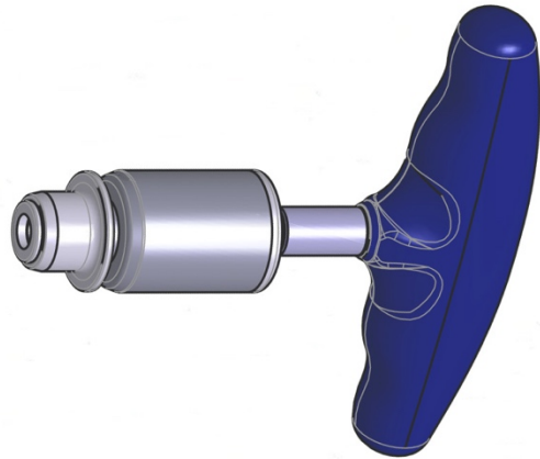
OM 23-0430 T23 Handle 1/4" Square Connect Torque Limiting - 12Nm 121.5mm Length
